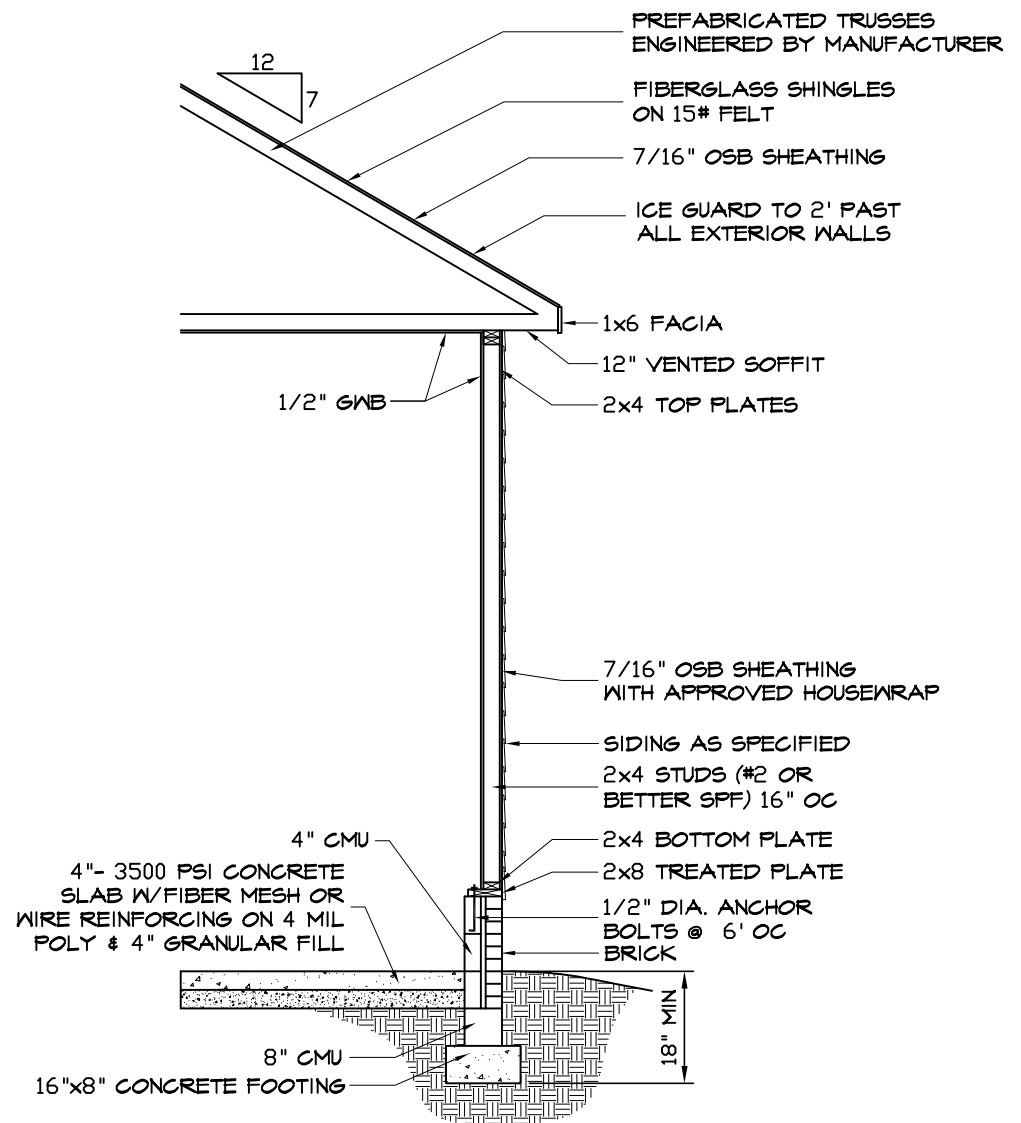
GARAGE WALL SECTION (TYP.)
