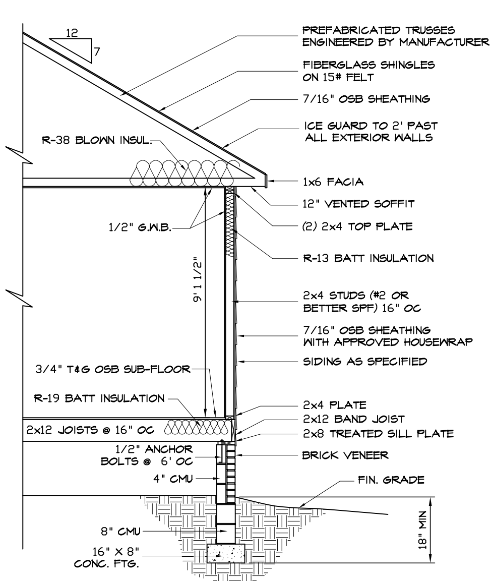
WALL SECTION (TYP.)
