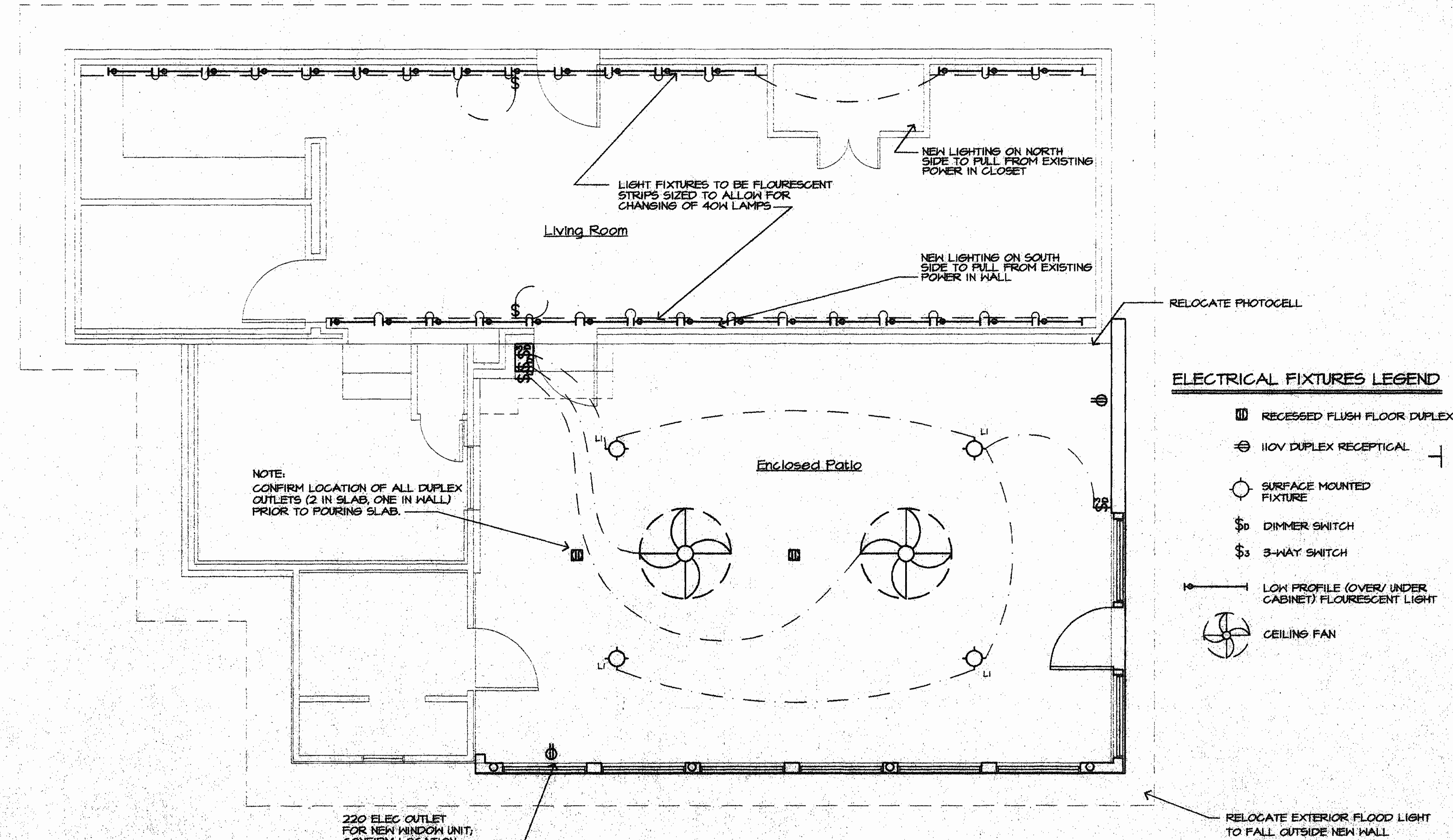
7 ELECTRICAL PLAN SCALE: 1/4"
