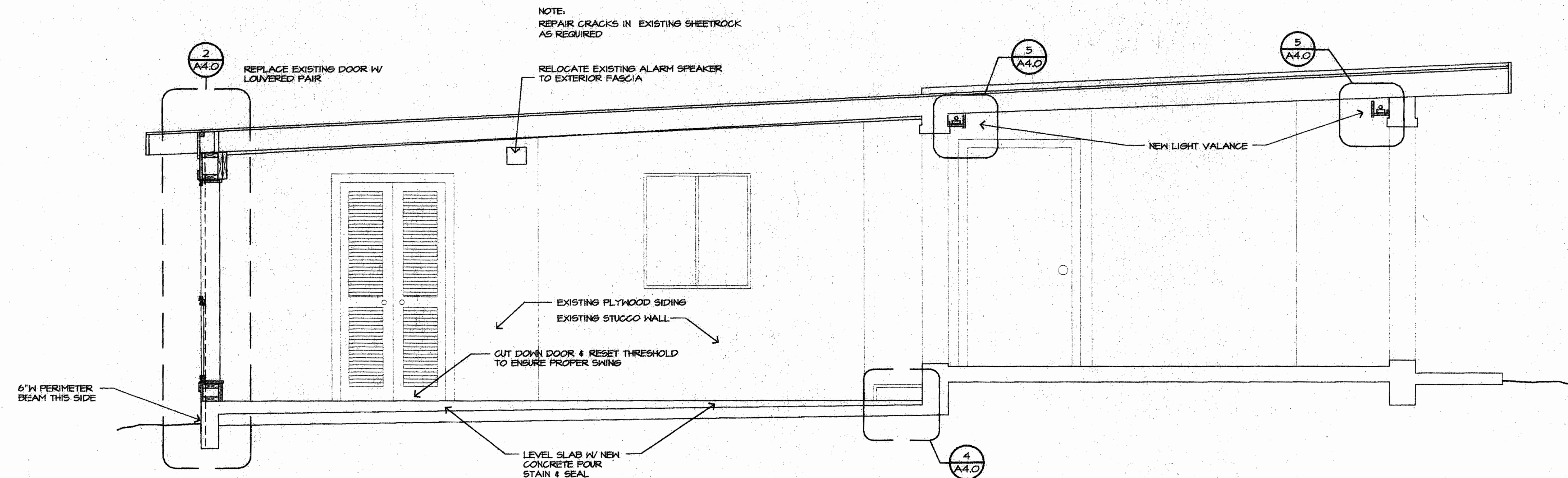
1 BUILDING SECTION SCALE: 1/2"
