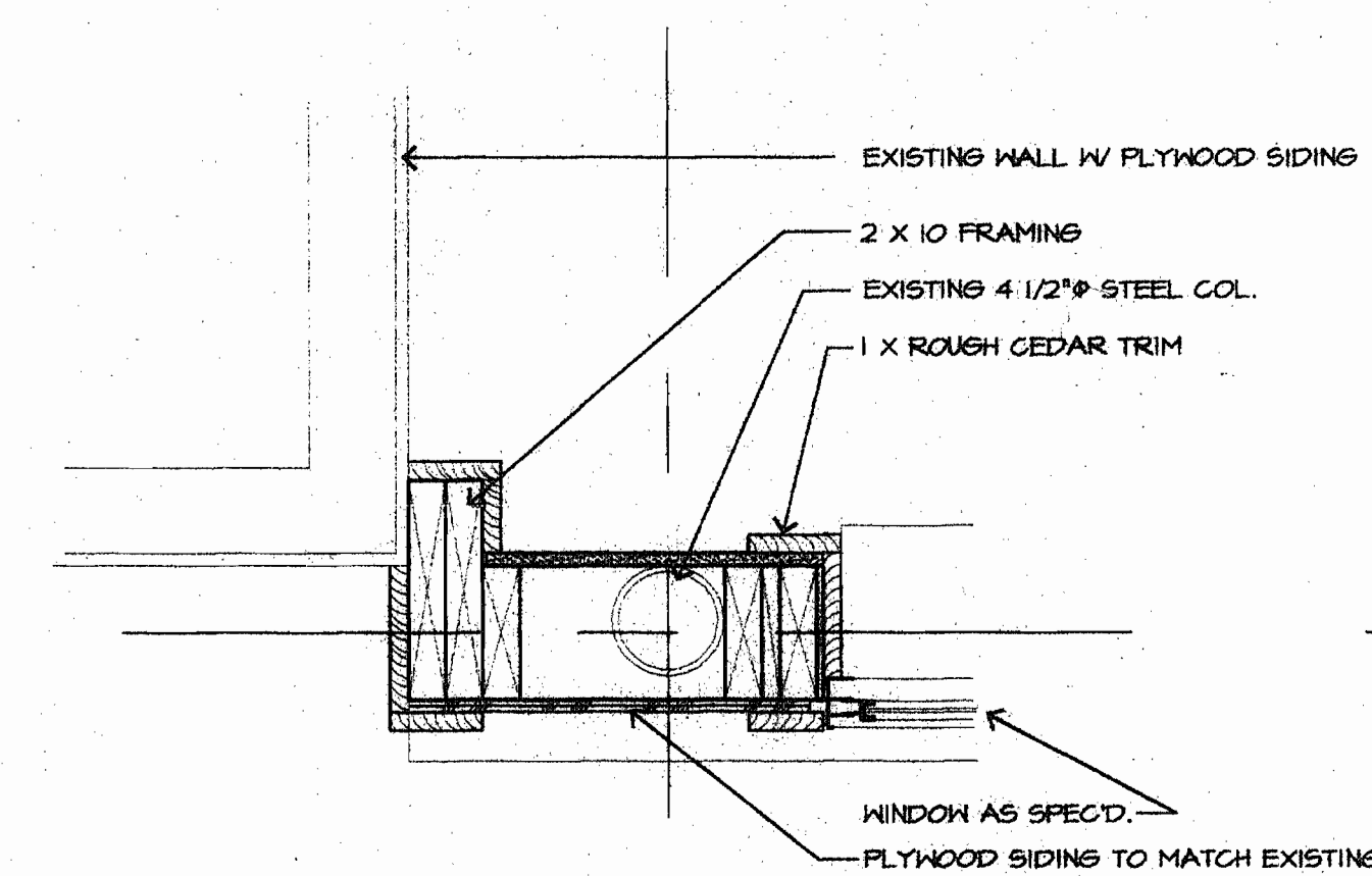
4 NEW TO EXIST. STUD WALL SCALE: 1 1/2"
