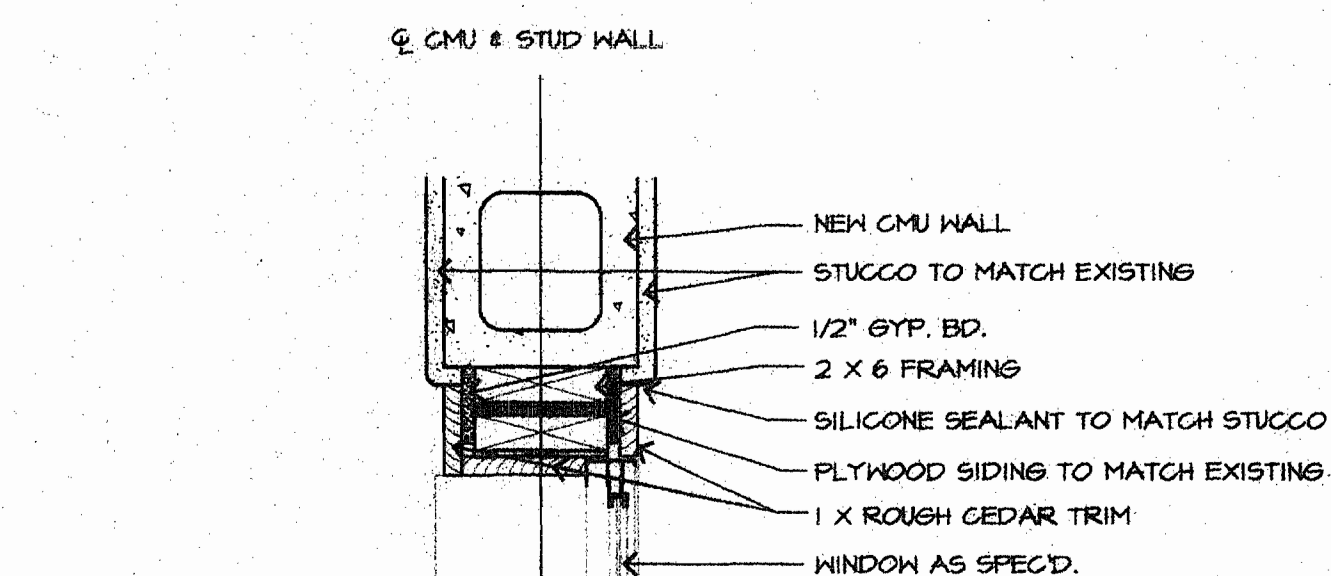
3 CMU TO NEW STUD WALL / JAMB SCALE: 1 1/2"
