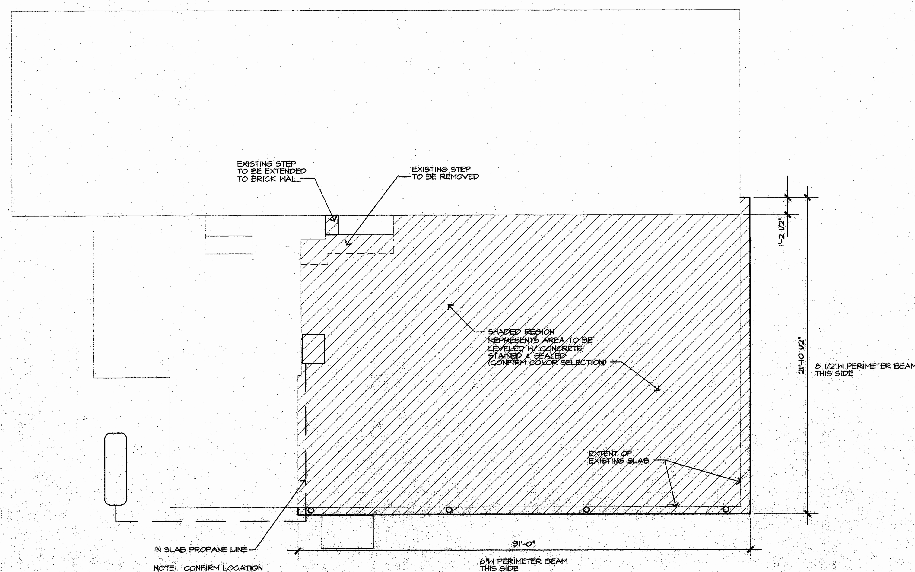
6 STRUCTURAL PLAN SCALE: 1/4"
