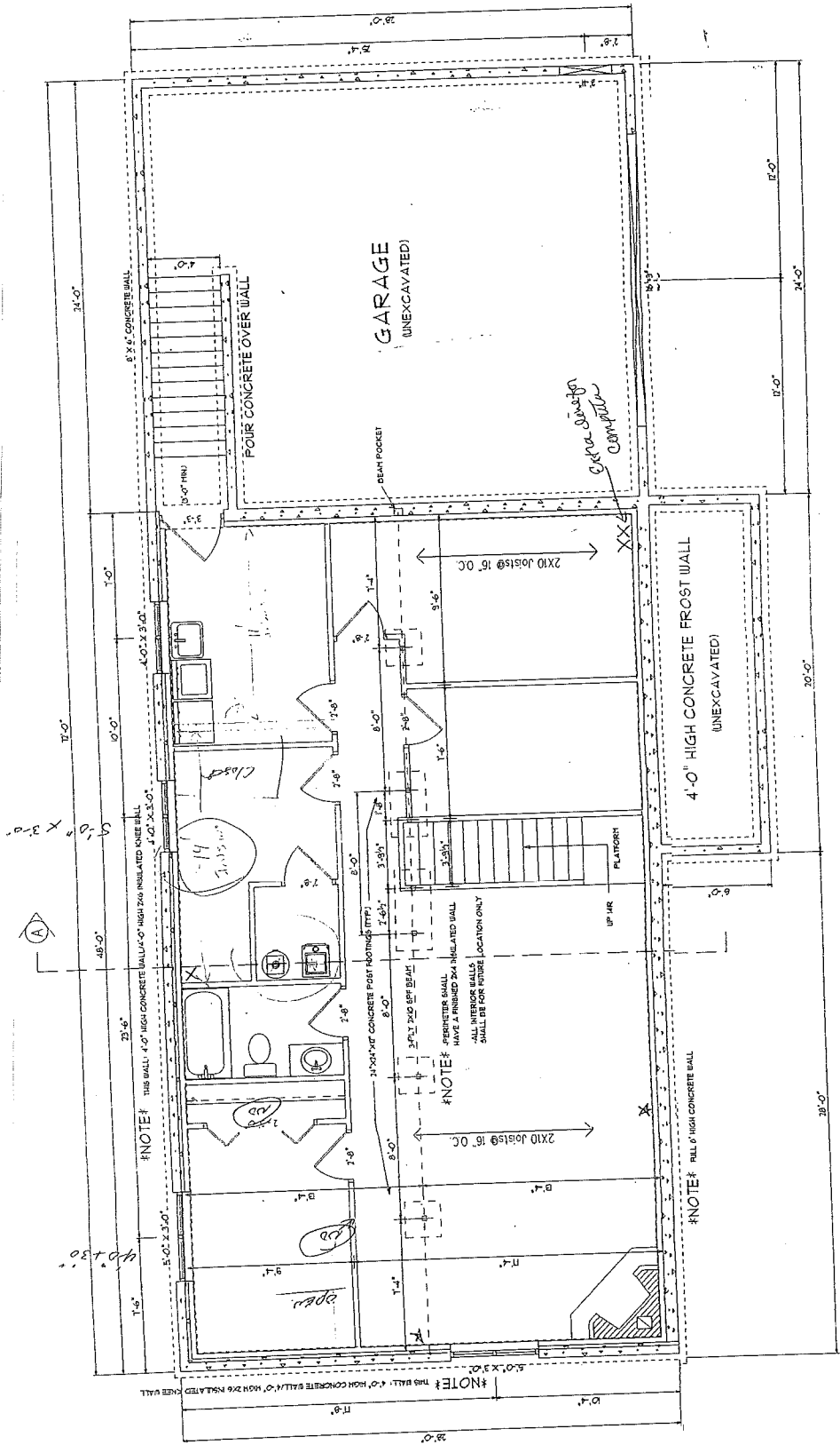
FOUNDATION LAYOUT
