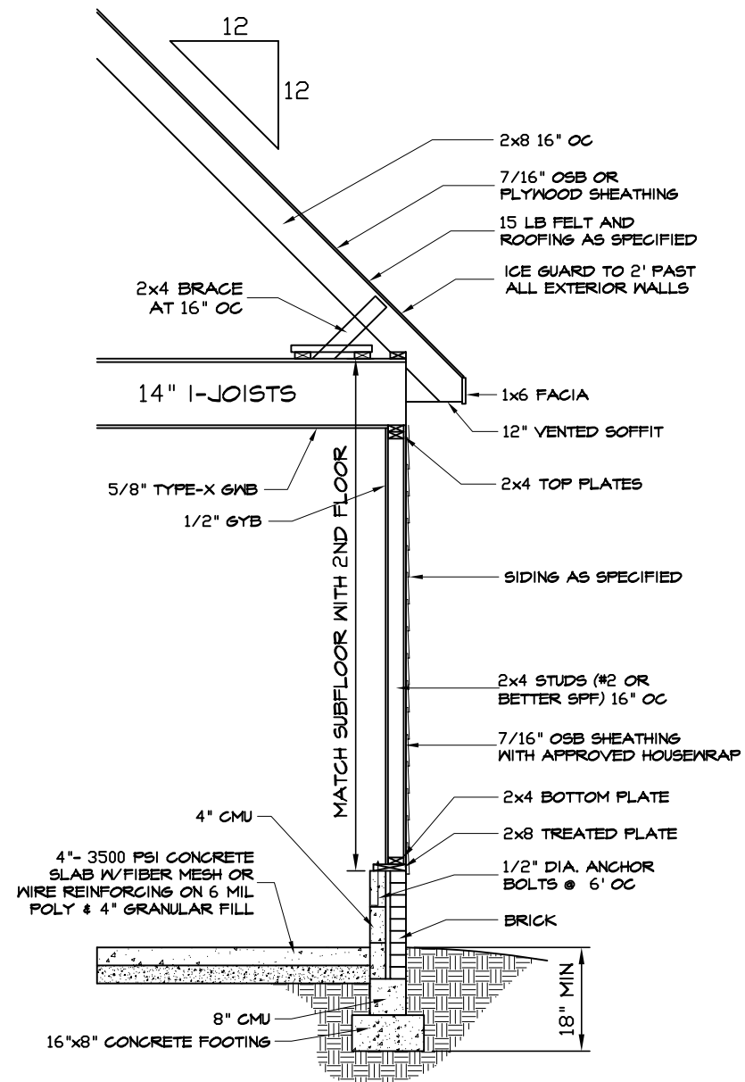
GARAGE WALL SECTION (TYP.)
