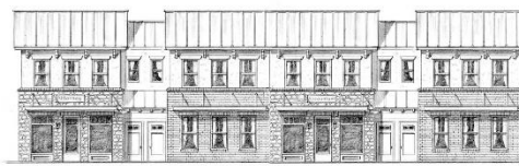
STREET ELEVATION - "SHOP HOUSES"
