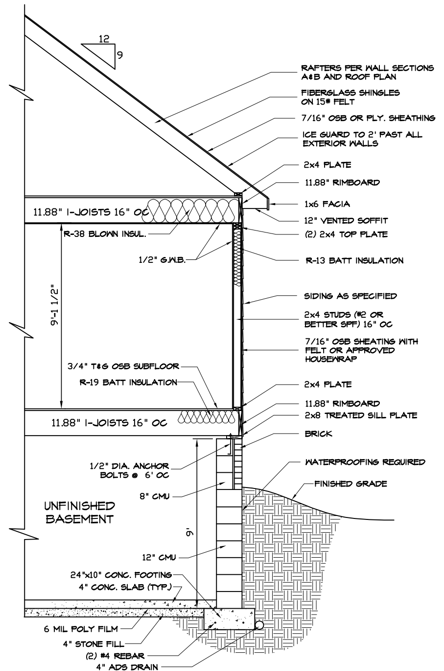
WALL SECTION (TYP.)
