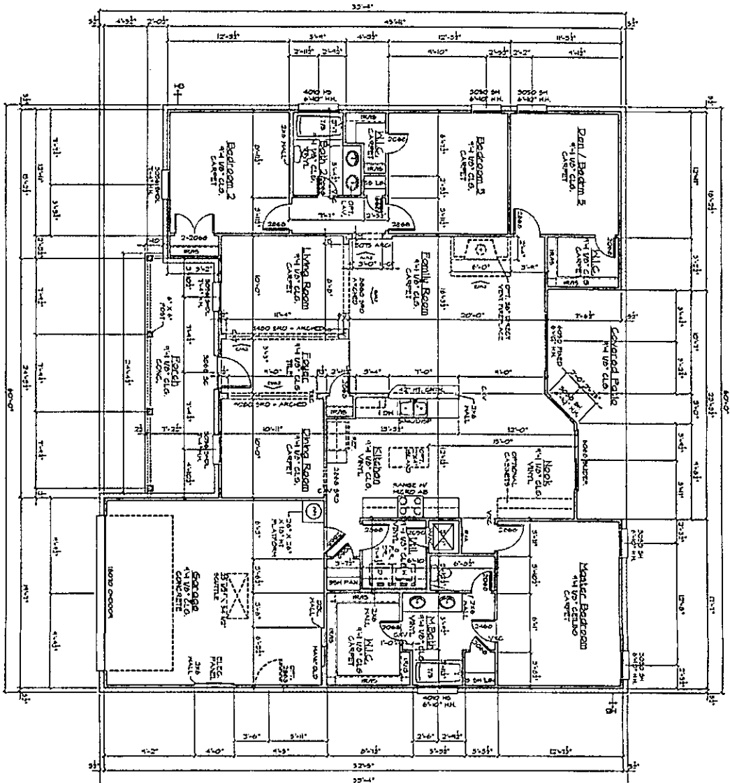
FLOOR PLAN
