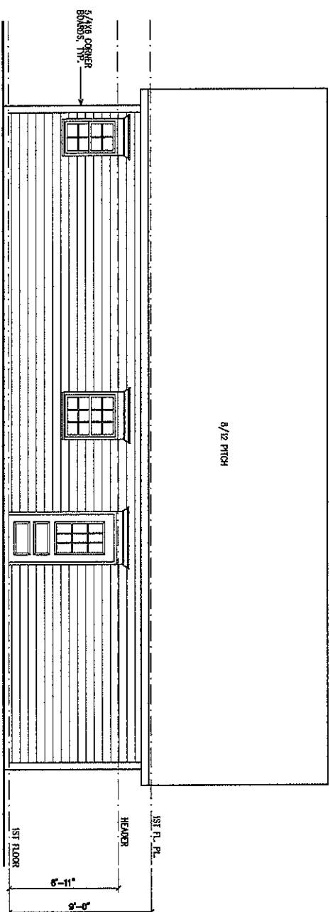
3/2 REAR ELEVATION
