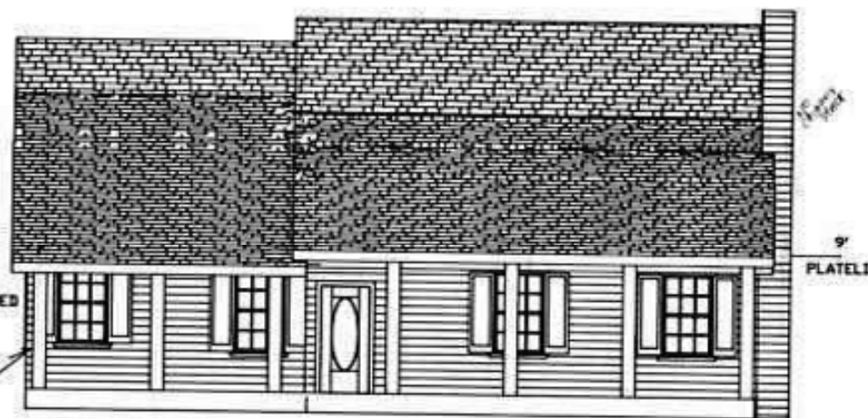
FRONT ELEVATION
