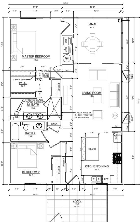
2 BEDROOM FLOOR PLAN
