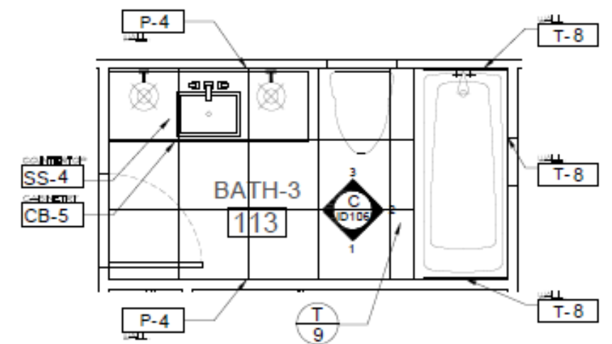
FLOOR PLAN BATH - 03
