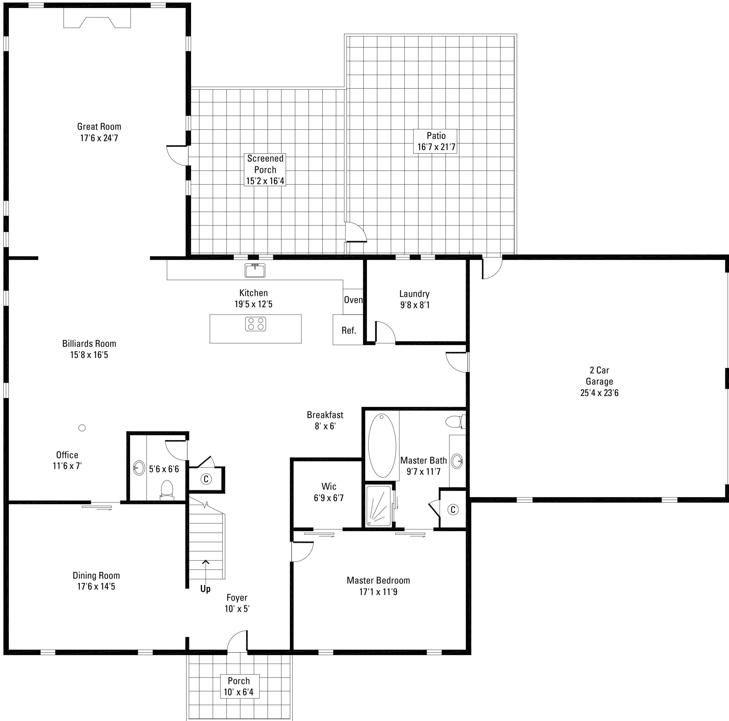
FIRST FLOOR
