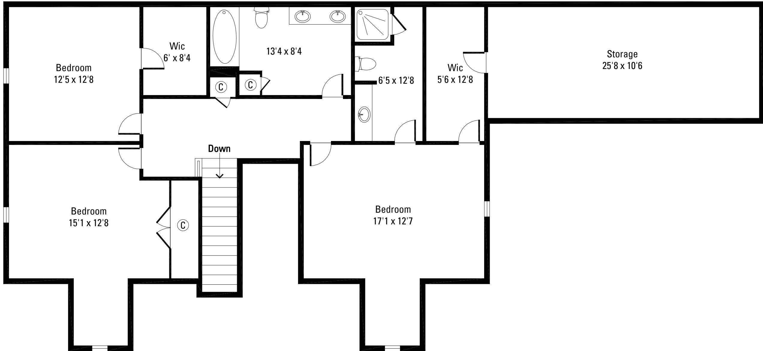
SECOND FLOOR
