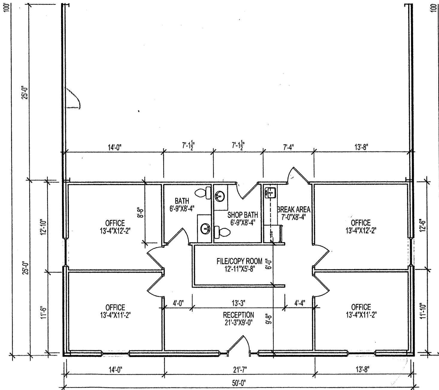
A FLOOR PLAN A-2.0 1/8"=1'-0"
