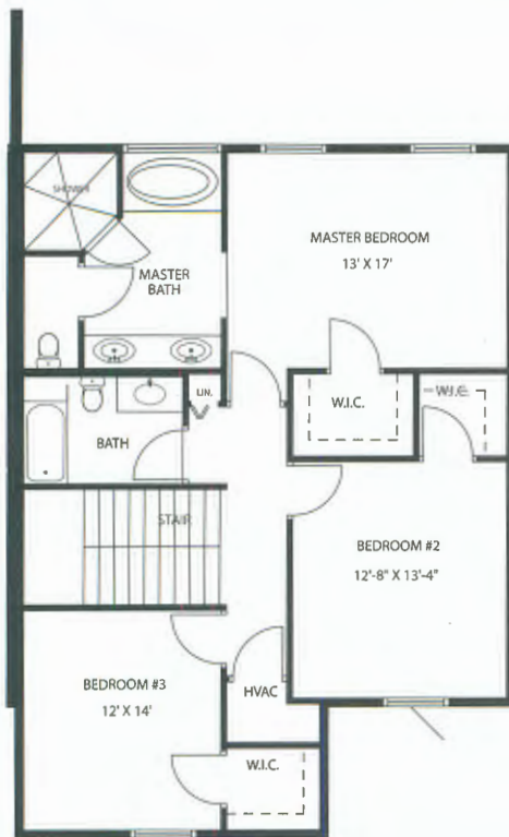
UNIT C SECOND FLOOR PLAN 1170 SQ. FT. L.A.
