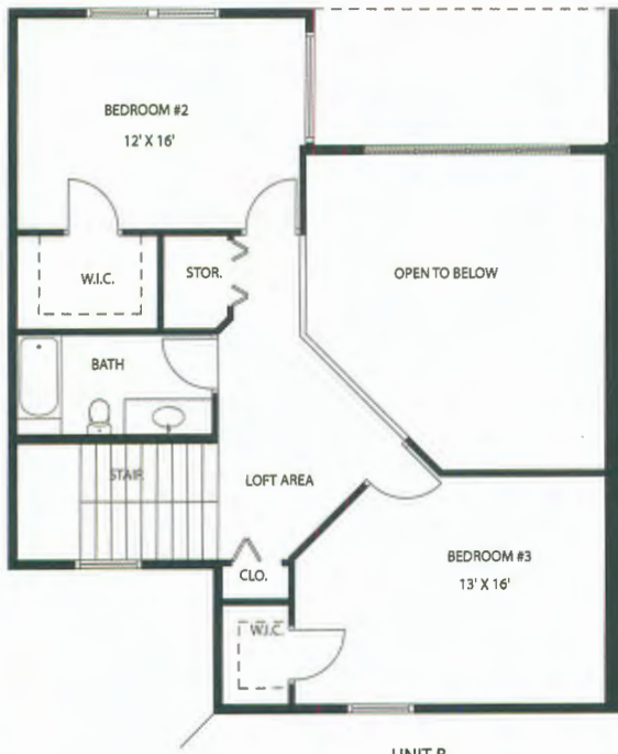
UNIT B SECOND FLOOR PLAN 935 SQ. FT. L.A.
