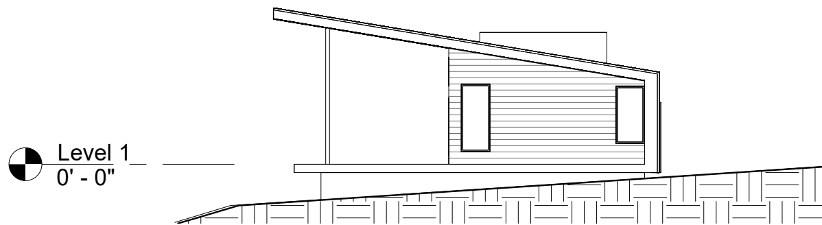
④ West 1/16" = 1'-0"
