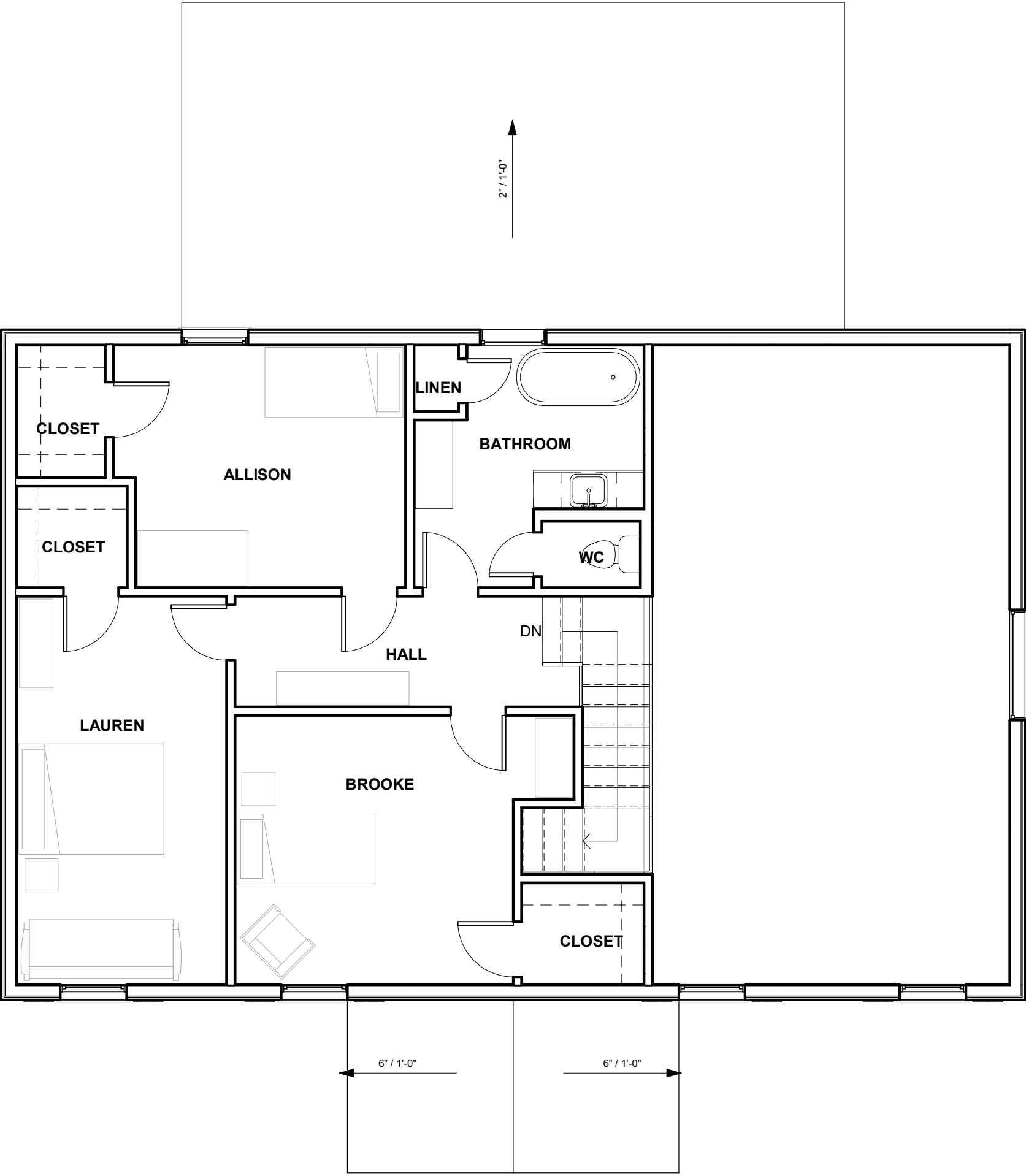
② Level 2 Furniture 3/16" = 1'-0"
