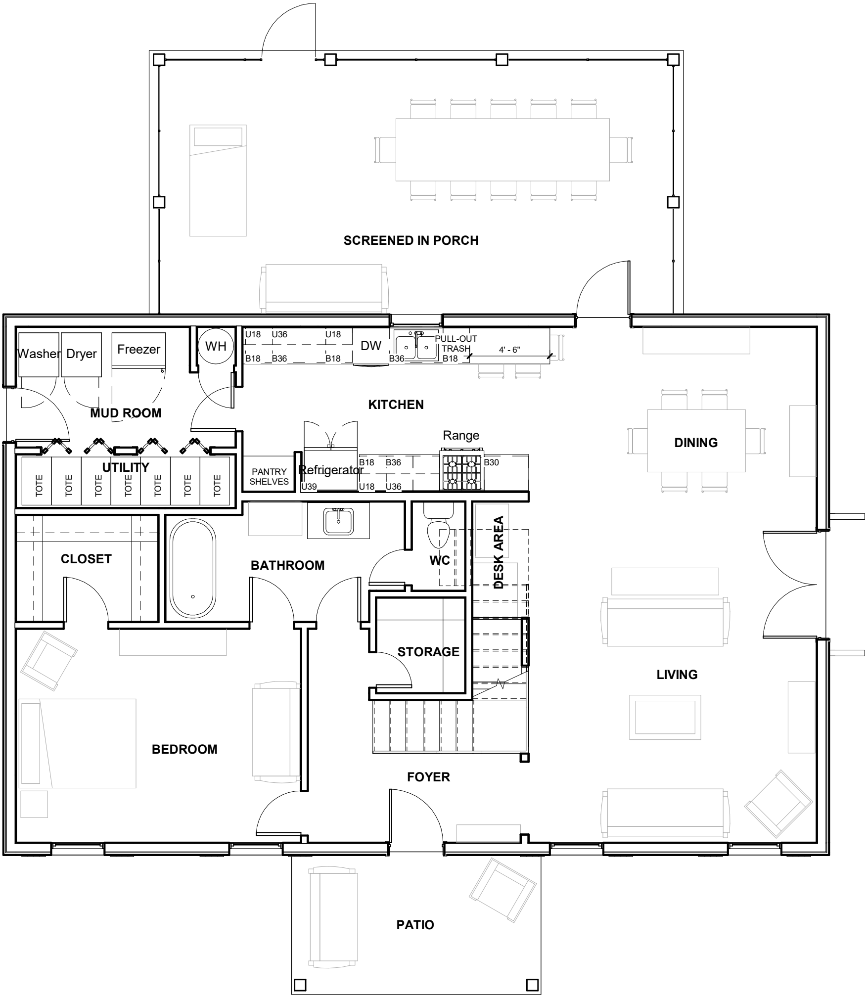
① Level 1 Furniture 3/16" = 1'-0"
