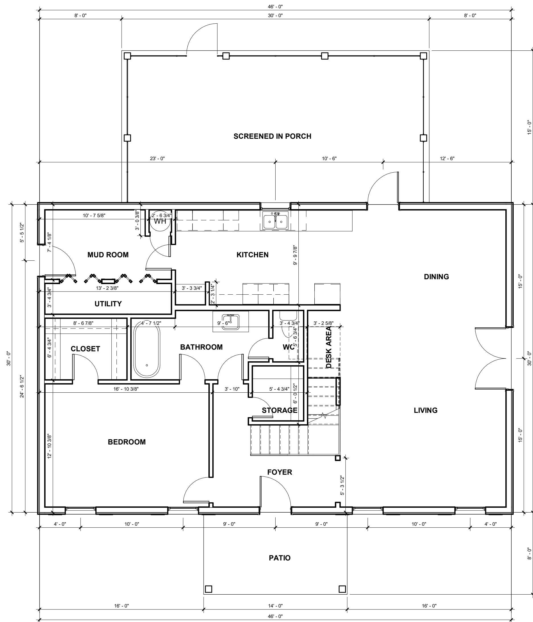
1 Level 1 Dimension 3/16" = 1'-0"
