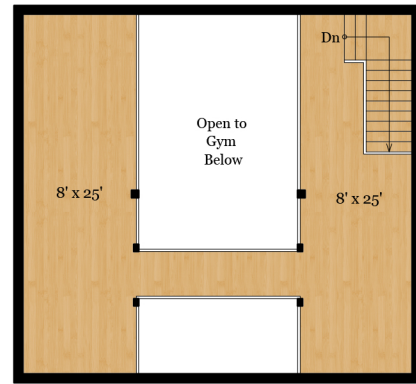
POOL HOUSE/GYM THIRD FLOOR 488 SQ FT - Finished
