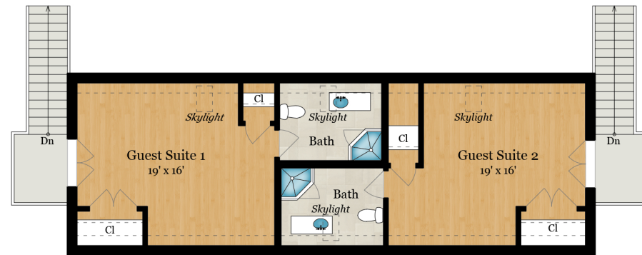
4-CAR GARAGE/GUEST SUITE 1 & 2 SECOND FLOOR 356 SQ FT - Finished (Guest Suite 1) 355 SQ FT - Finished (Guest Suite 2) 197 SQ FT - Unfinished & Usable
