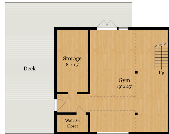
POOL HOUSE/GYM SECOND FLOOR 739 SQ FT - Finished
