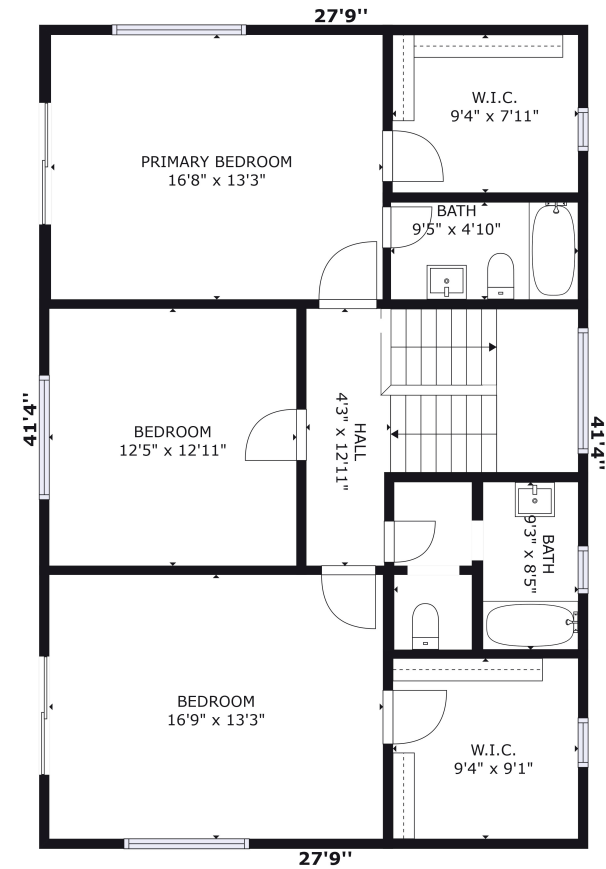
MAIN HOUSE FLOOR 2
