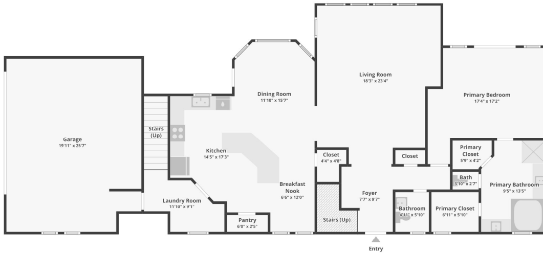
FLOOR 1
