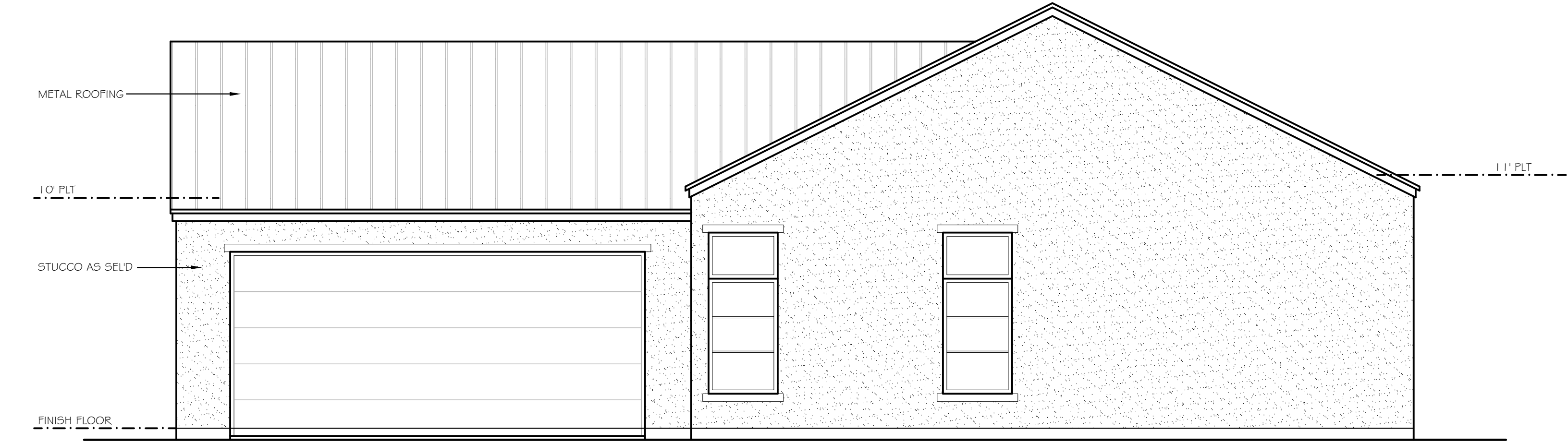
LEFT ELEVATION
